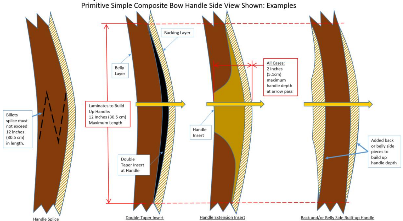
Figure 4 Primitive Simple Composite Bow Handle Examples
