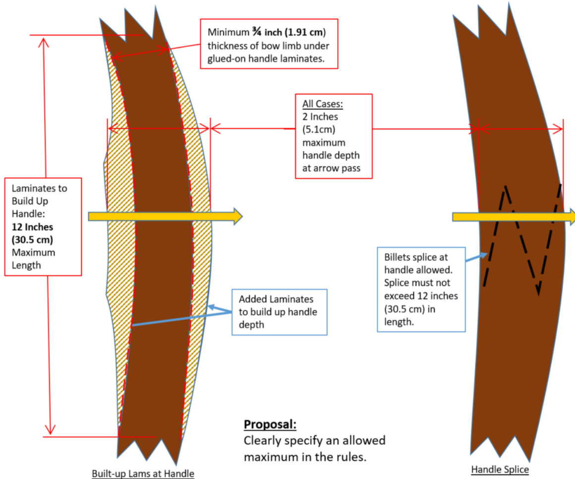
Figure 3 - Self Bow Handle Examples
